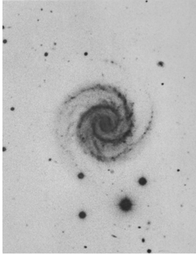
1 NGC 2857 (M) p. 220
