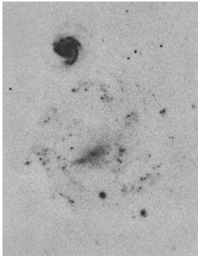
4 MCG-2-5-50 and companion (H) p. 180
