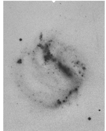
5 NGC 3664 (W) p. 330
