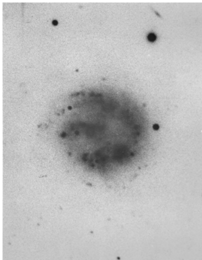
6 NGC 2537, The Bearpaw (M) p. 221
